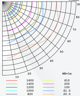
PLANAR ISOLUX DIAGRAM (UNIT: 1X)
