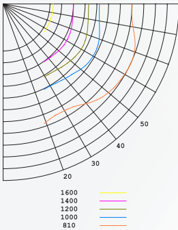
PLANAR ISOLUX DIAGRAM (UNIT: 1X)
