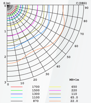
PLANAR ISOLUX DIAGRAM (UNIT: 1X)
