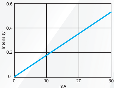
BRIGHTNESS/CURRENT CHARACTERISTICS CURVE
