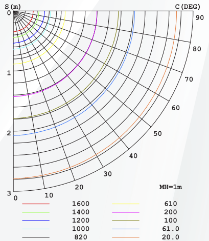
PLANAR ISOLUX DIAGRAM (UNIT: lx)
