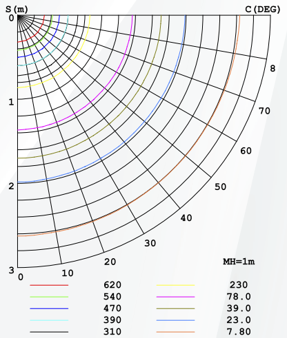
PLANAR ISOLUX DIAGRAM (UNIT: 1X)
